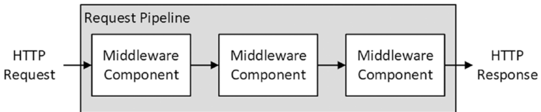
Figure 12-2. The ASP.NET Core request pipeline
