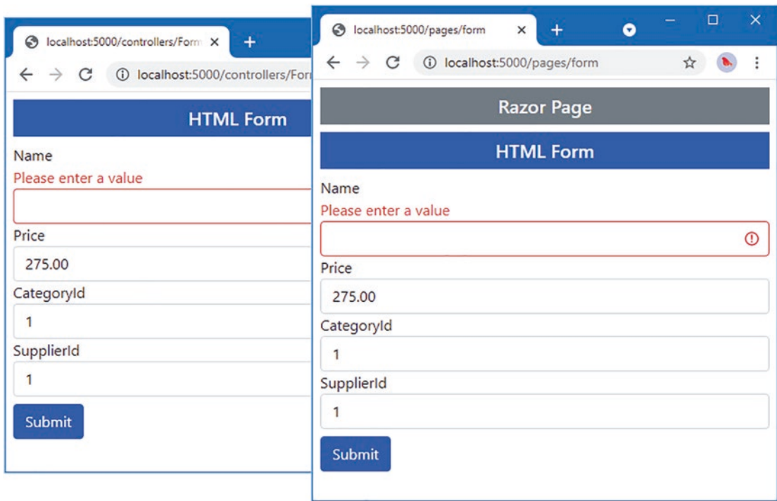
Figure 29-11. Using custom validation attributes
