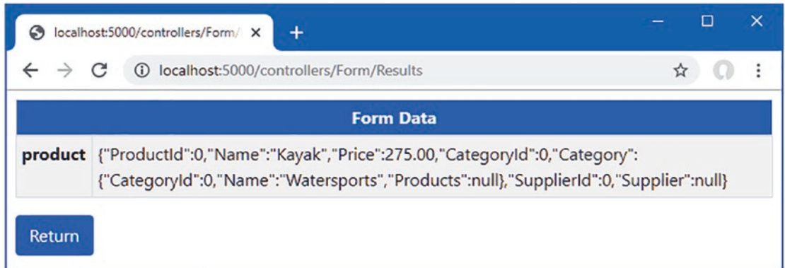
Figure 28-9. Model binding a nested property
