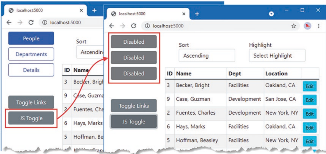
Figure 35-13. Invoking a component method from JavaScript
