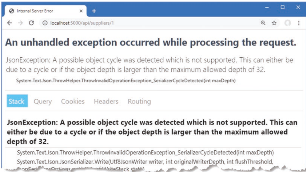
Figure 20-2. An exception caused by querying for related data
