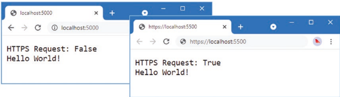
Figure 16-7. Detecting an HTTPS request
