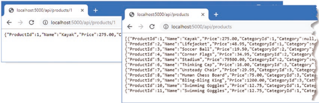
Figure 19-2. Web service response
