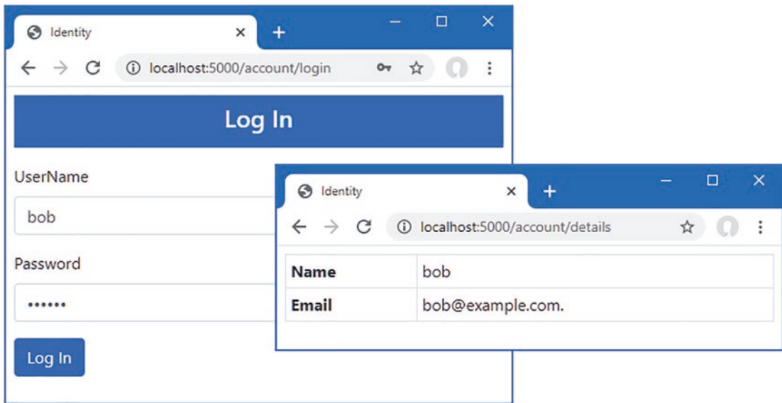
Figure 39-4. Getting details of an authenticated user
