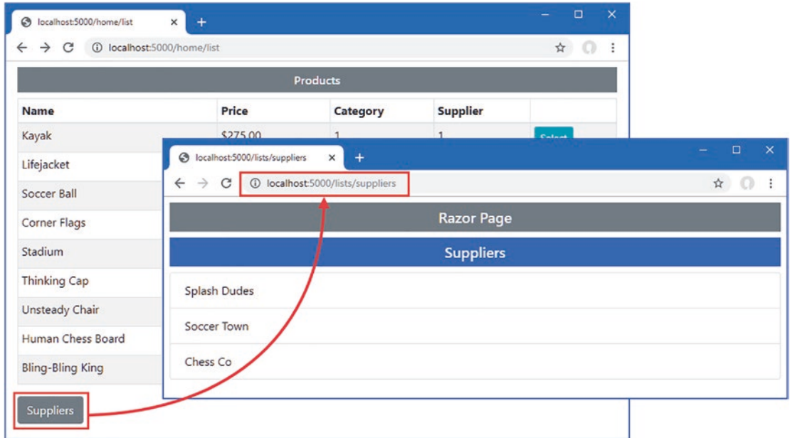
Figure 26-4. Targeting a Razor Page with an anchor element
