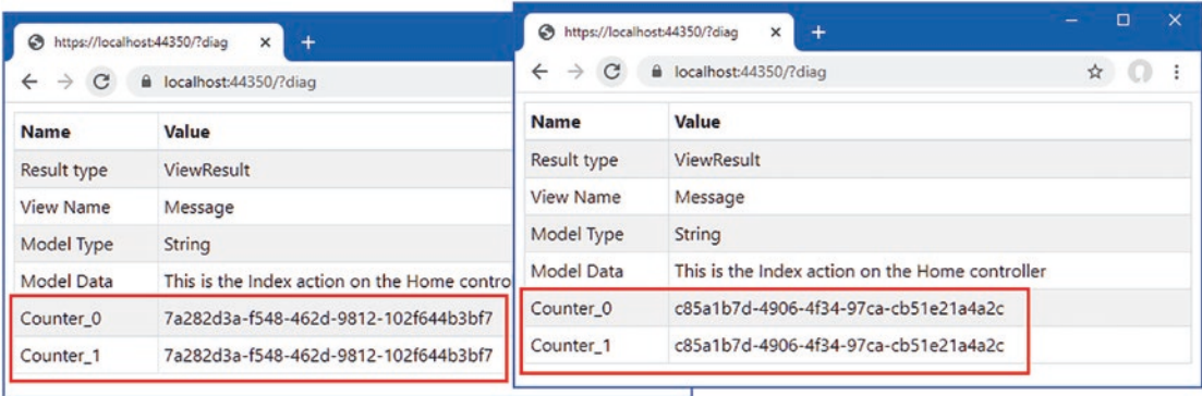
Figure 30-14. Using dependency injection to manage filters
