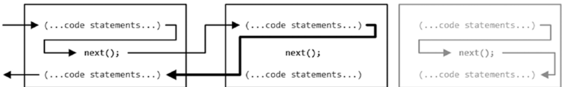
Figure 12-10. Short-circuiting the request pipeline
