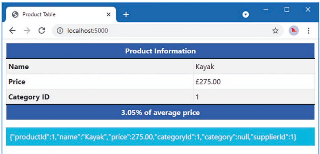
Figure 22-17. Encoding an expression result as JSON
