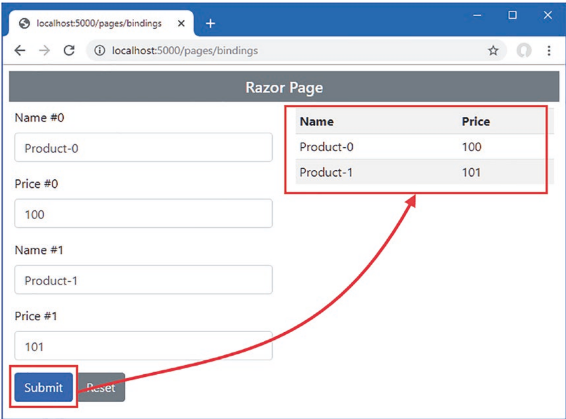
Figure 28-18. Binding to a collection of complex types
