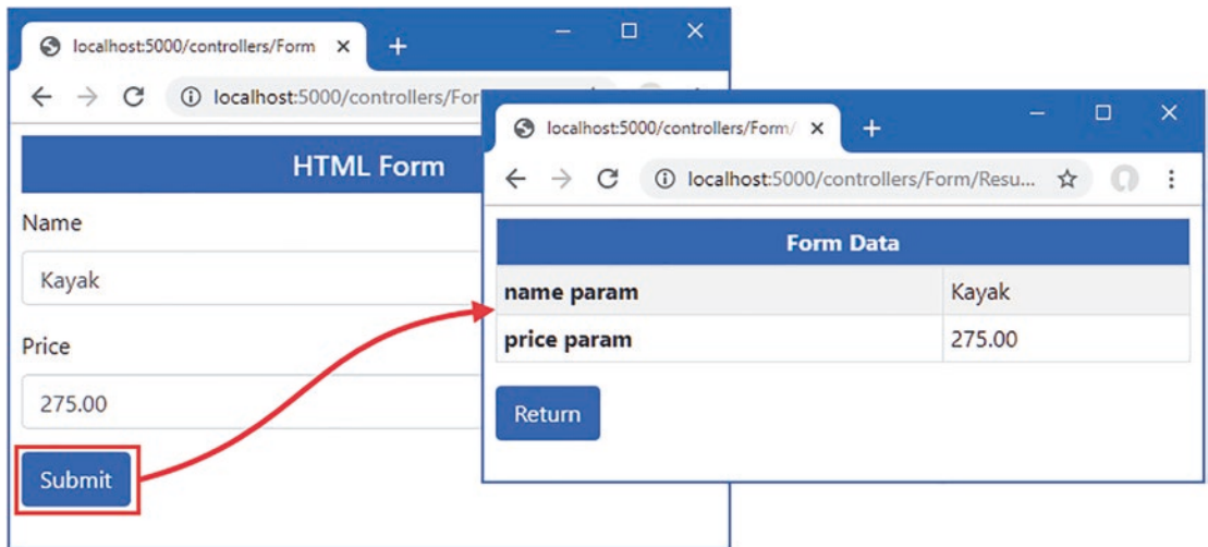
Figure 28-3. Model binding for simple types
