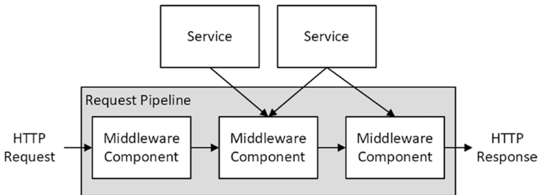
Figure 12-3. Services in the ASP.NET Core platform
