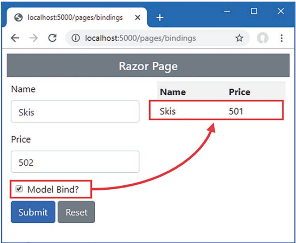
Figure 28-21. Using manual model binding
