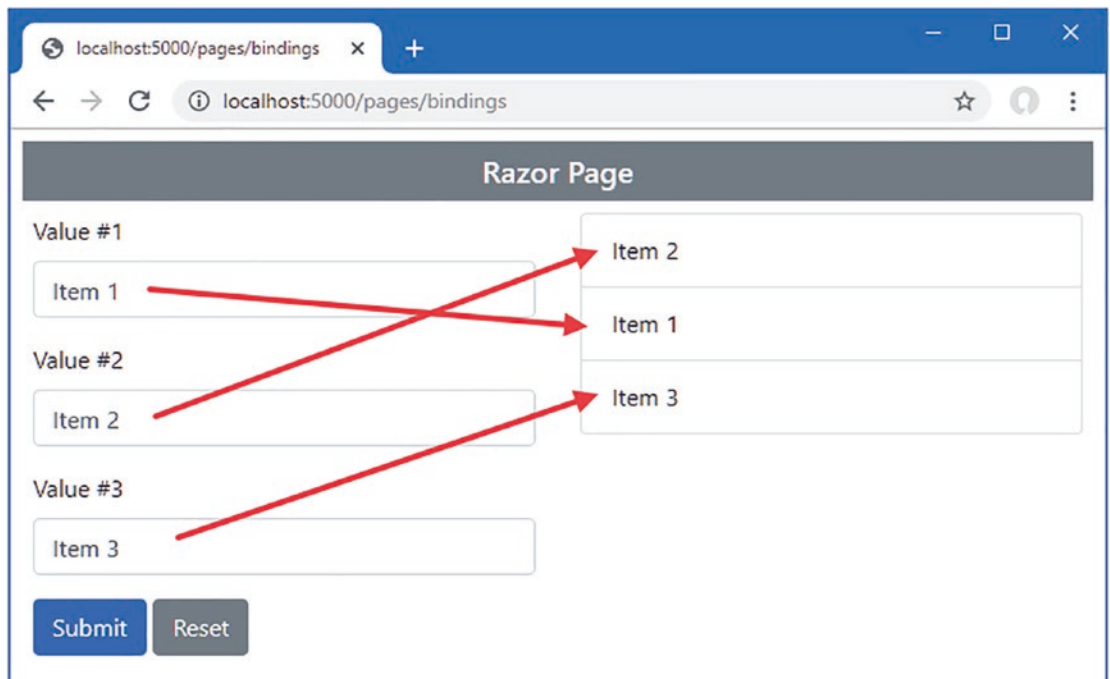
Figure 28-15. Specifying array position
