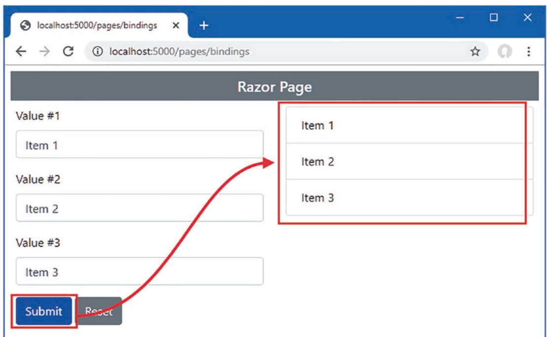
Figure 28-14. Model binding for array values
