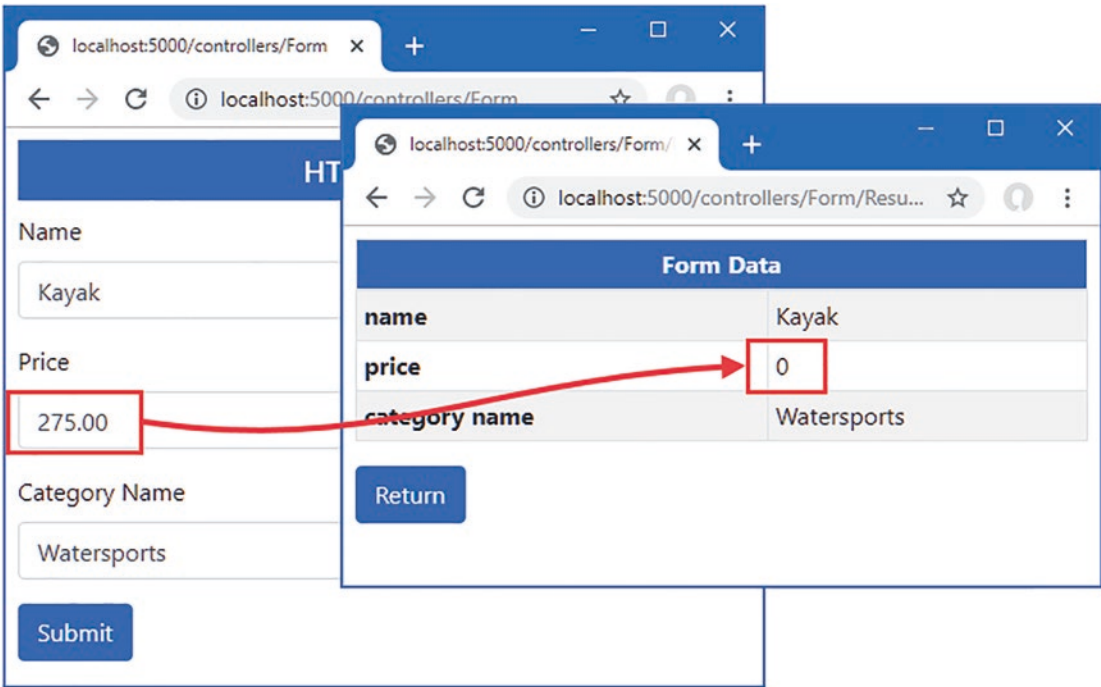
Figure 28-12. Selectively binding properties
