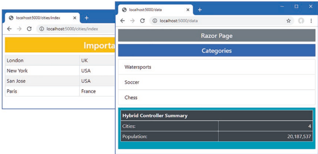
Figure 24-13. A hybrid controller and view component class
