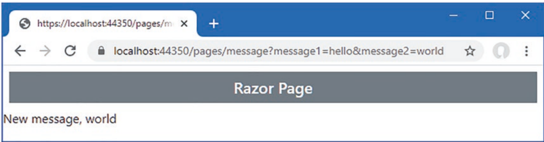
Figure 30-9. Using a page filter
