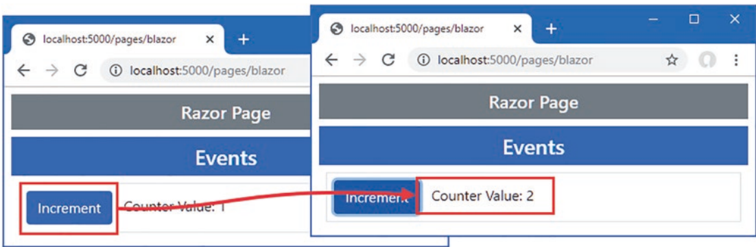
Figure 33-6. Handling an event
