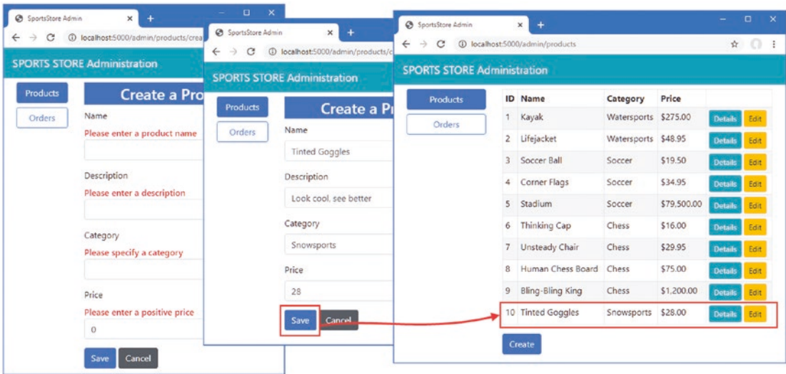
Figure 10-7. Using the Editor component
