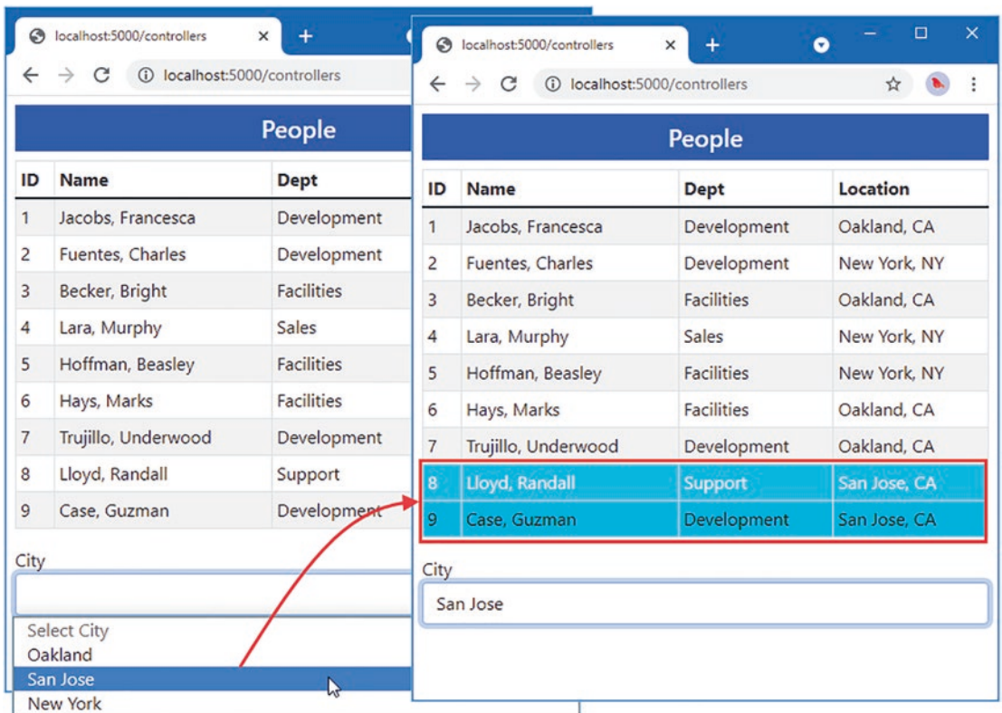
Figure 33-4. Using a Razor Component
