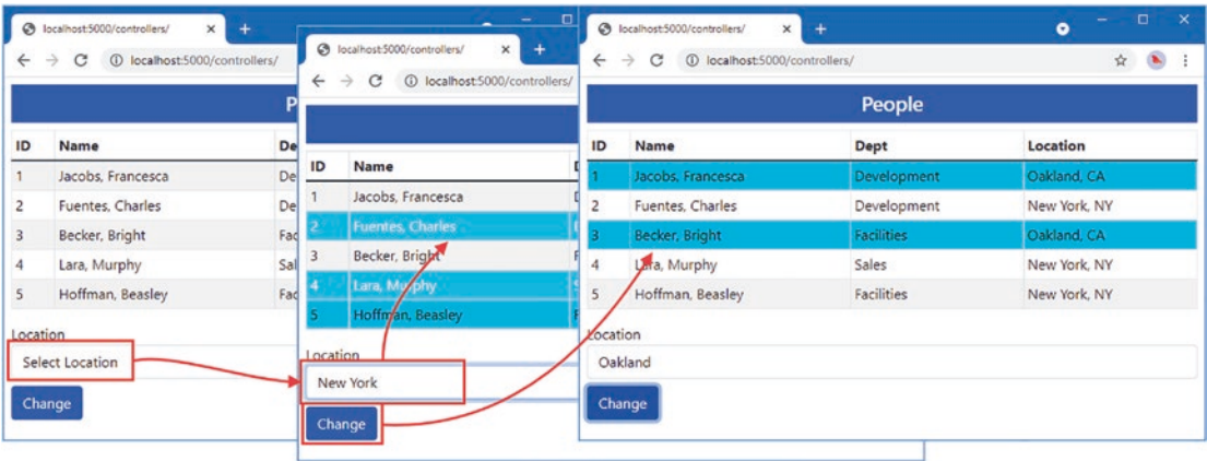
Figure 34-5. Using a custom binding
