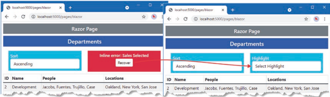
Figure 34-16. Recovering from an error
