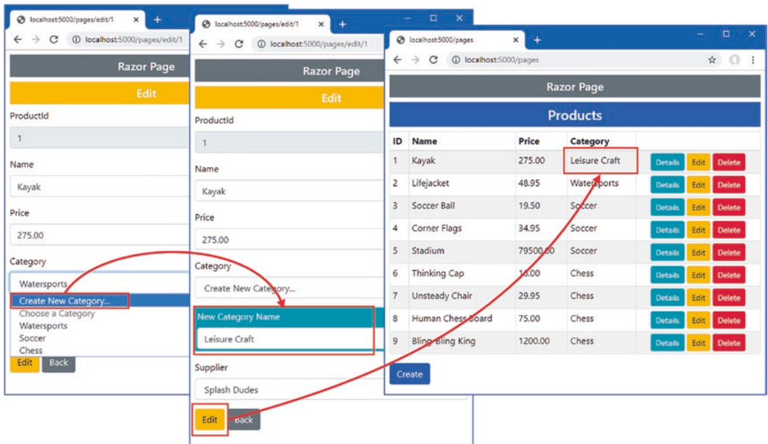
Figure 31-9. Creating related data
