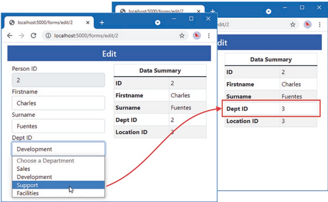
Figure 36-3. Using a custom form element
