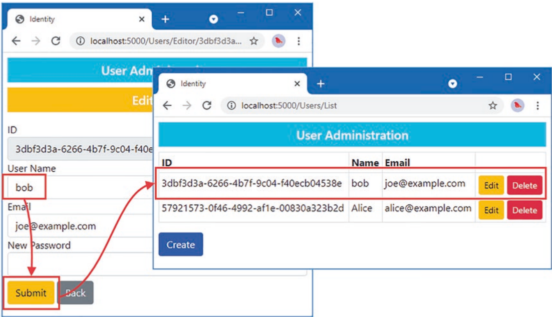
Figure 38-9. Editing a user
