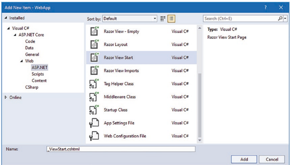
Figure 22-7. Creating a view start file
