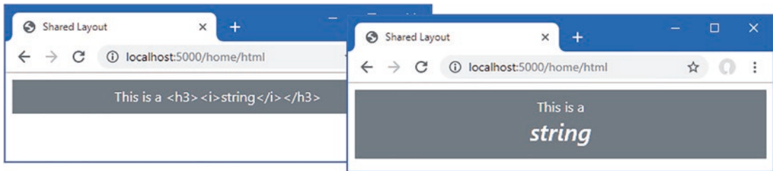
Figure 22-16. HTML result encoding
