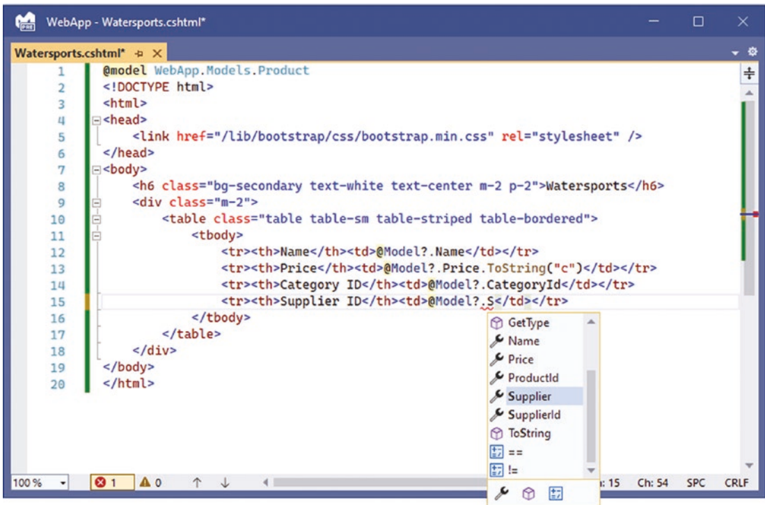
Figure 21-10. Editor suggestions when using a view model type
