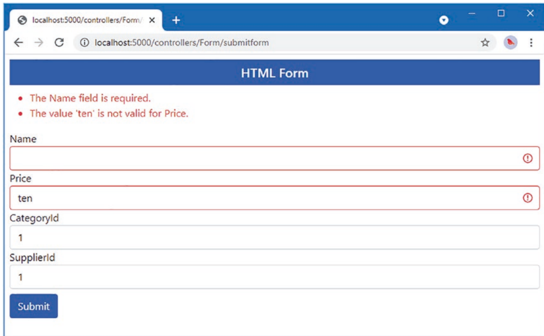
Figure 29-4. Displaying a parsing validation message
