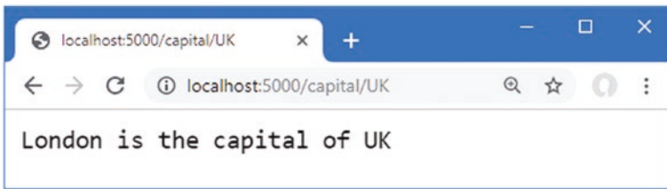
Figure 13-18. Matching specific values with a regular expression
