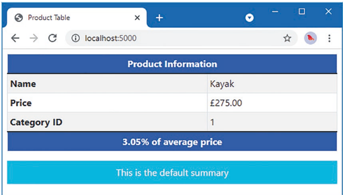
Figure 22-13. Displaying fallback content for a view section
