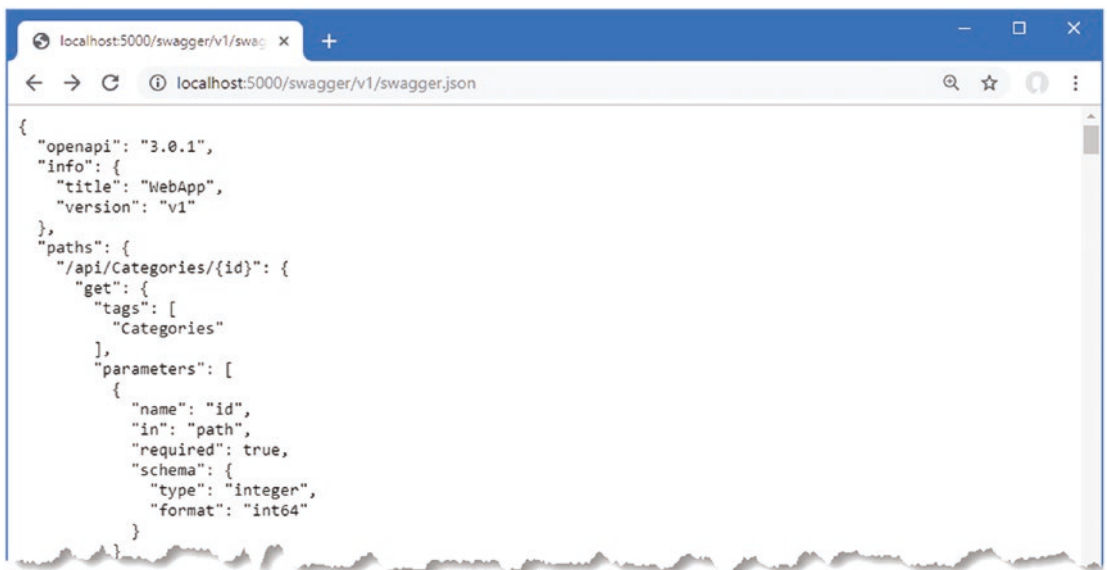
Figure 20-7. The OpenAPI description of the web service
