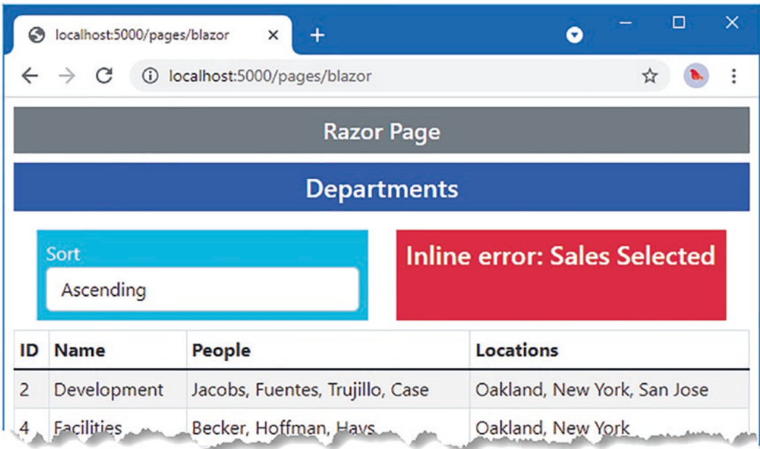
Figure 34-15. Error content defined within the boundary
