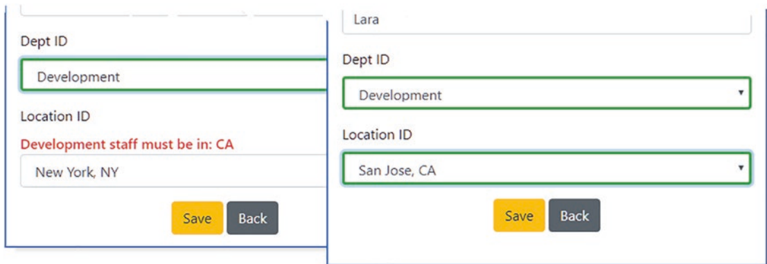
Figure 36-12. Creating a custom validation component
