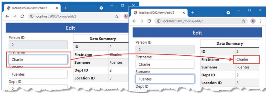
Figure 36-2. Using the Blazor form elements
