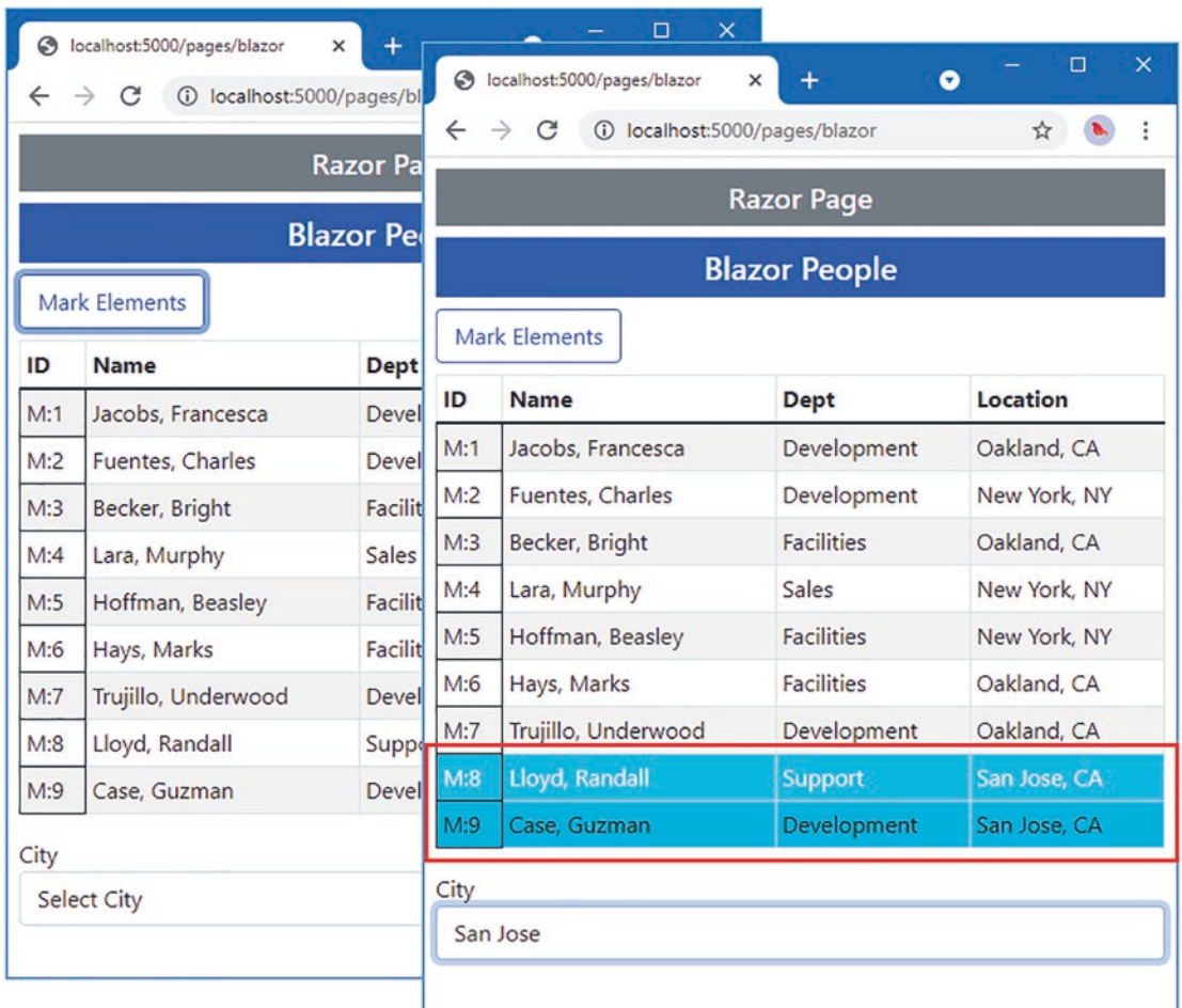
Figure 33-5. Demonstrating that only changes are used
