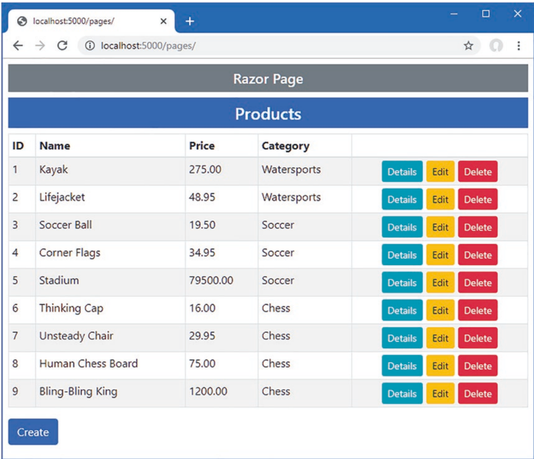
Figure 31-7. Listing data using a Razor Page
