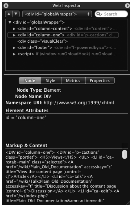
Figure 4-6. The built-in DOM inspector in Safari
