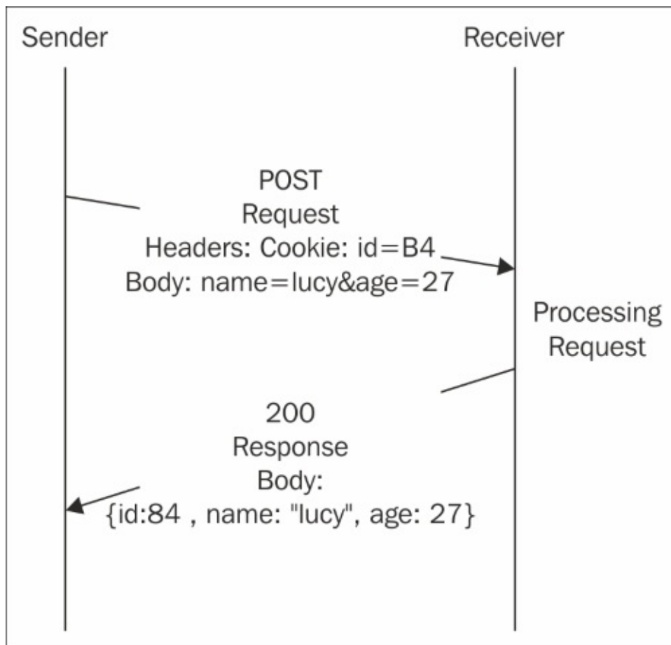
A more complex POST request
