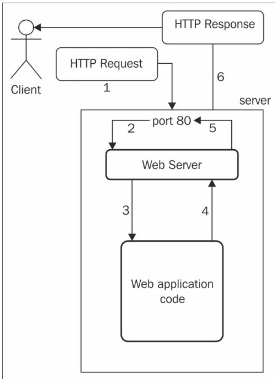
Request-response flow on the server side
